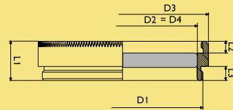
SN2 Rotating Mount: Filter thickness 1.0 - 4.5 mm
