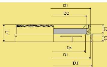
HST Mount: Filter thickness 1.3 - 2.2 mm
