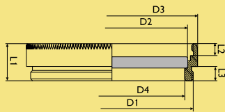
SN1 Mount: Filter thickness 1.0 - 4.0 mm
