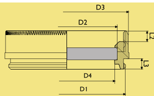
DH Mount: Filter thickness 2.2 - 4.5 mm
